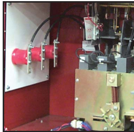
High voltage compartment (including vacuum contactor, main fuses, motor connection bus and mechanical emergency run mechanism).
